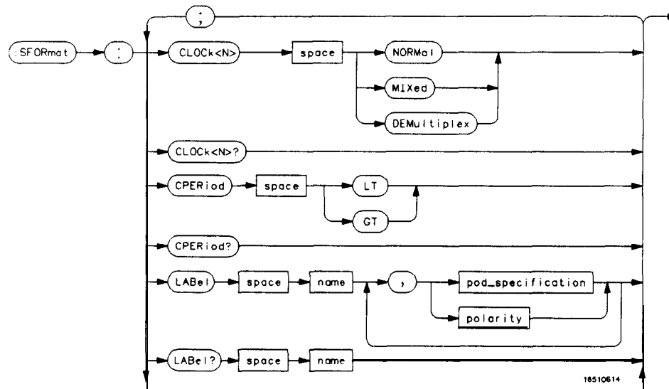
Figure 1 I-I. SFORmat Subsystem Syntax Diagram
